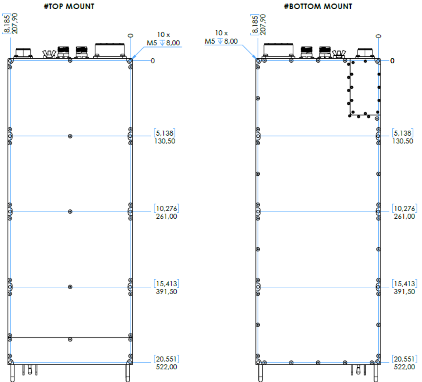
Figure 29. Mounting Details and Mounting Holes Coordinates
