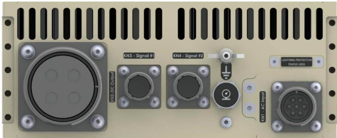
Figure 18. Connector Panel
