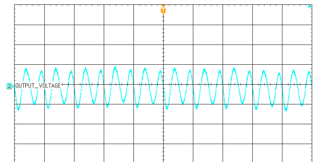
Output voltage (blue) (100 mV/div) Time base: 10 μs/div
